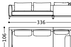
01BOWC8 (1BOW220SX + 1BOW281DX) 02BOWC8 (2BOW220SX + 2BOW281DX)
