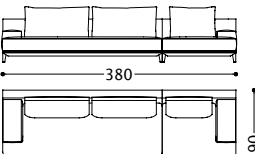
01RNNC10 (1RNN230SX + 1RNN281DX) 02RNNC10 (2RNN230SX + 2RNN281DX)
