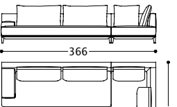
01RNNC10 (1RNN230SX + 1RNN281DX) 02RNNC10 (2RNN230SX + 2RNN281DX)
