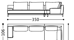
01RNNC11 (1RNN230SX + 1RNN260DX) 02RNNC11 (2RNN230SX + 2RNN260DX)
